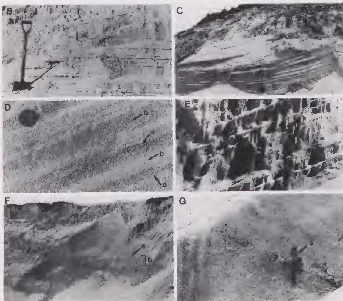
Figure 2 Range of stratification features at a single typical locality, Banjup West. See Fig. 1 for location. A Panoramic diagram of stratification and location of insets. B A large scale, tabular set of planar horizontal strata overlain by a large scale, wedge-shaped set of planar cross-strata (inclined strata). C A large scale set of concave-upwards, trough cross-strata. Note the rivulets of flowing sand which are building avalanche cones of sand. The continued growth of avalanche cones of sand will eventually conceal the stratification. D Thinnest recognizable strata in a large-scale set of low angle, planar cross-strata produced by differences in grain size of framework sand grains. The coarser layers (a) resemble ripple-form strata of Hunter (1977). The finer layers (b) resemble grainfall strata of Hunter (1977). Coin is 21mm in diameter. E Layering in a large-scale set of planar cross-strata produced by differences in texture, composition and colour. Thin prominent layers have framework quartz-sand grains supported in a silt-clay matrix of yellowish brown goethite, kaolin and quartz. Thick layers lack the silt-clay matrix. Coin is 28mm in diameter. F Discontinuity (a) between two units of yellow sand. The discontinuity between the units is produced by: geometry of interface; changes in stratification details away from the contact; and structural, textural, compositional and colour differences between the two units on either side of the interface. The massive zone below the discontinuity is a palaeosol (b) which indicates the discontinuity is a regional bounding surface (Talbot 1985). Note also the common indistinct appearance of stratification. Several metres of surficial sand has been removed from this section by excavating machinery. Spade for scale is 1 m in length. G Closer view of disconformity surface, sloping from upper left to lower right and with underlying, mostly massive palaeosol with rare organic material and burrow-structures (a). Note rivulets of flowing sand on the left hand side. Coin is 24 mm in diameter.
